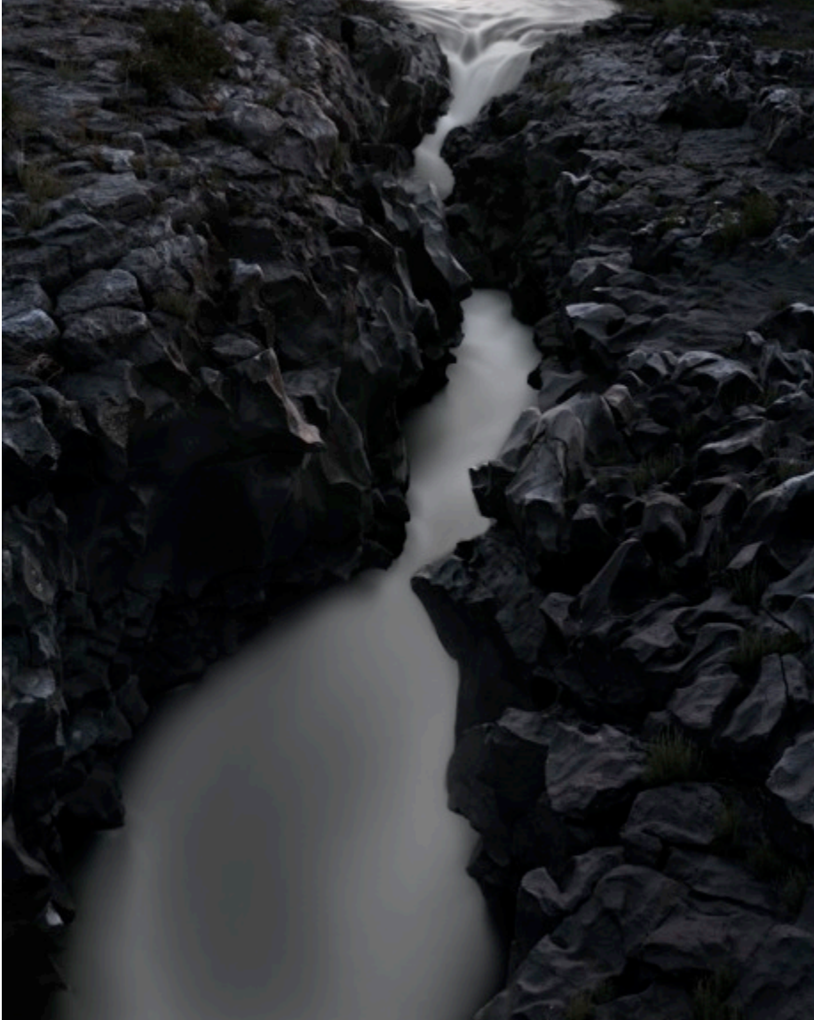
Big Wood River Crossing A Lava Flow, Lincoln County, Idaho 2017
